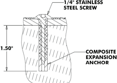
EXPANSION ANCHOR DETAIL (ASPHALT)
