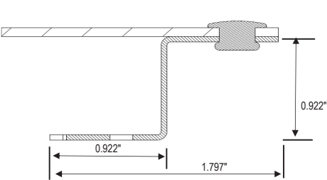
WET-SET, Z-BRACKET ANCHOR DETAIL (FRESH CONCRETE)
