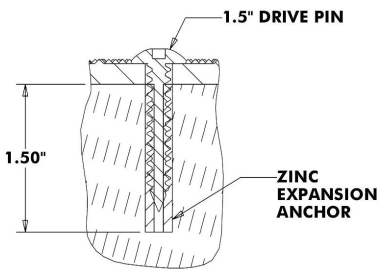
EXPANSION ANCHOR DETAIL (HARDENED CONCRETE)
