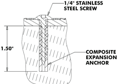
EXPANSION ANCHOR DETAIL (ASPHALT)
