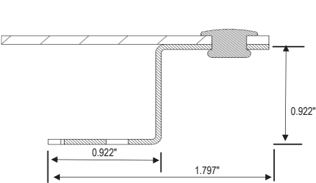
WET-SET, Z-BRACKET ANCHOR DETAIL (FRESH CONCRETE)
