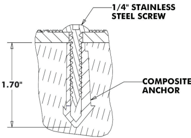
WET SET ANCHOR DETAIL (FRESH CONCRETE)
