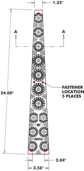
RADIUS - WEDGE TILE
