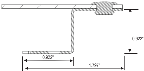
WET-SET, Z-BRACKET ANCHOR DETAIL (FRESH CONCRETE)
