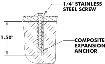
EXPANSION ANCHOR DETAIL (ASPHALT)
