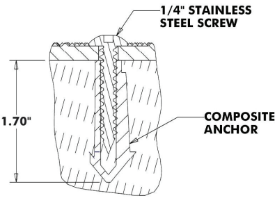
WET SET ANCHOR DETAIL (FRESH CONCRETE)
