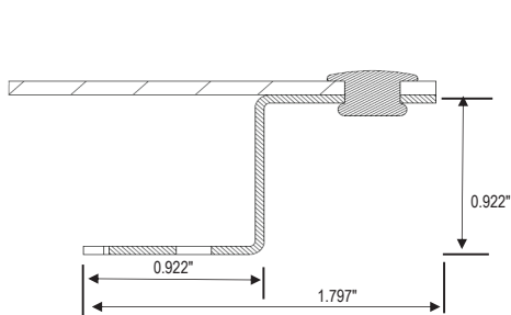
WET-SET, Z-BRACKET ANCHOR DETAIL (FRESH CONCRETE)
