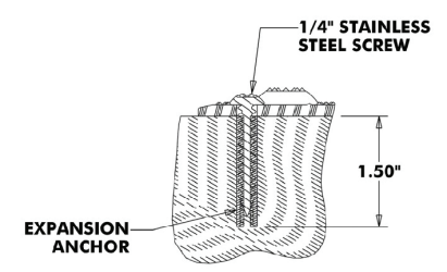
EXPANSION ANCHOR DETAIL (ASPHALT)
