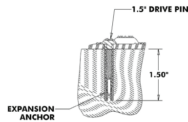
EXPANSION ANCHOR DETAIL (HARDENED CONCRETE)
