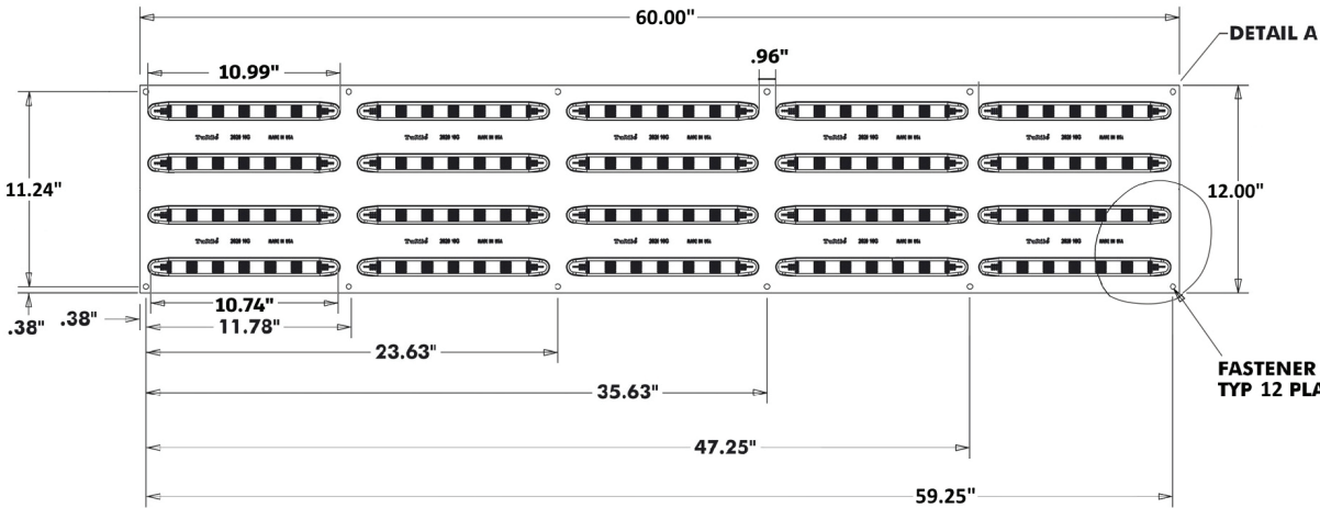
DETAIL A
