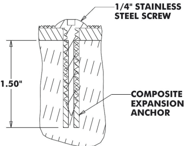
EXPANSION ANCHOR DETAIL (ASPHALT)
