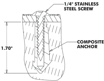
WET SET ANCHOR DETAIL (FRESH CONCRETE)
