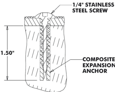
EXPANSION ANCHOR DETAIL (ASPHALT)
