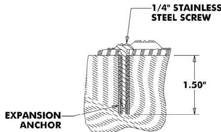
EXPANSION ANCHOR DETAIL (ASPHALT)
