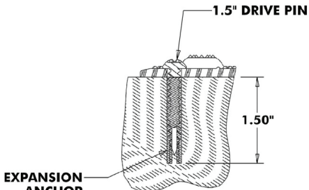
EXPANSION ANCHOR DETAIL (HARDENED CONCRETE)
