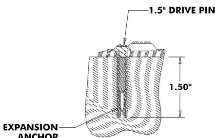
EXPANSION ANCHOR DETAIL (HARDENED CONCRETE)
