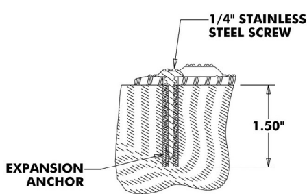
EXPANSION ANCHOR DETAIL (ASPHALT)
