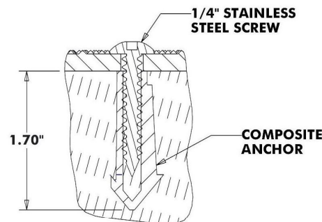
WET SET ANCHOR DETAIL (FRESH CONCRETE)
