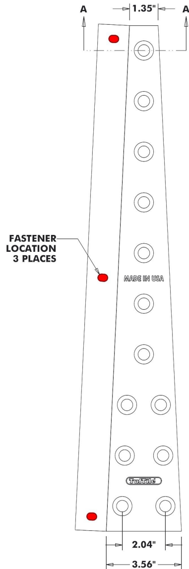
RADIUS - WEDGE TILE
