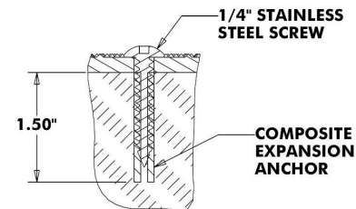
EXPANSION ANCHOR DETAIL (ASPHALT)
