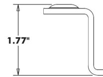
GV STEEL STIFFENER BAR END VIEW
