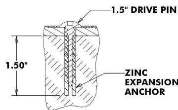
EXPANSION ANCHOR DETAIL (HARDENED CONCRETE)
