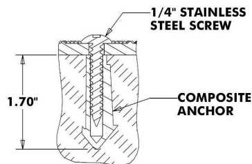
WET SET ANCHOR DETAIL (FRESH CONCRETE)
