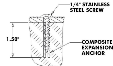
EXPANSION ANCHOR DETAIL (ASPHALT)
