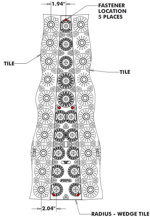
PLACEMENT VIEW
