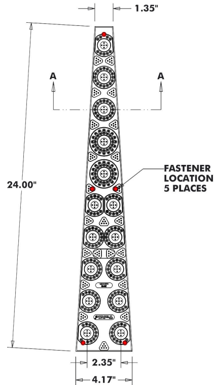
RADIUS - WEDGE TILE
