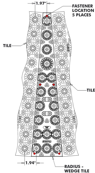
PLACEMENT VIEW
