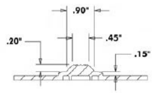
SECTION A
