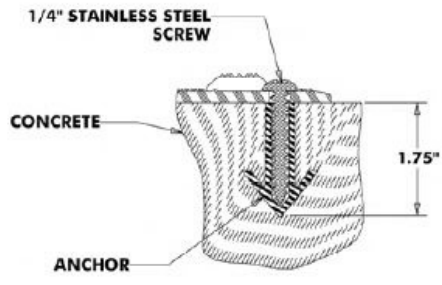
ANCHOR DETAIL
